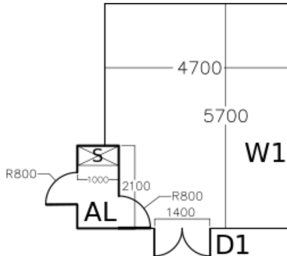
Figure 1: Cleanroom-1000 floor plan
