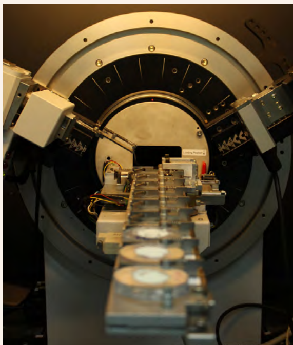
Bruker Powder Diffractometer
